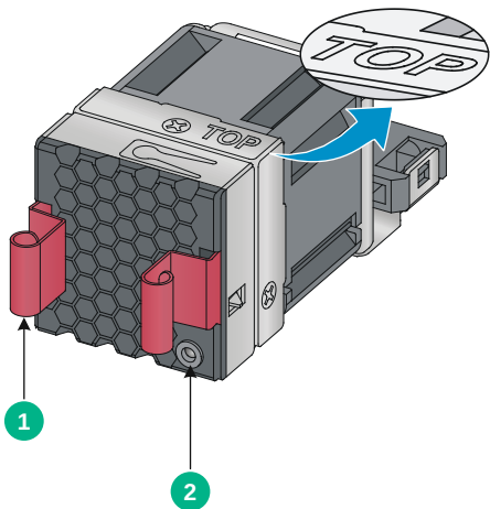
图2-12 LSPM1FANSB1-Z 风扇模块
